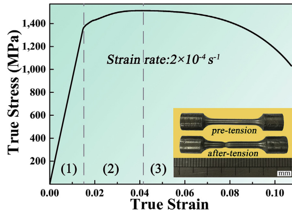
Fig. 2. Tensile true stress-true strain curve of the \text{Ti}_{50}\text{Zr}_{20}\text{V}_{10}\text{Cu}_5\text{Be}_{15} MGMC.
