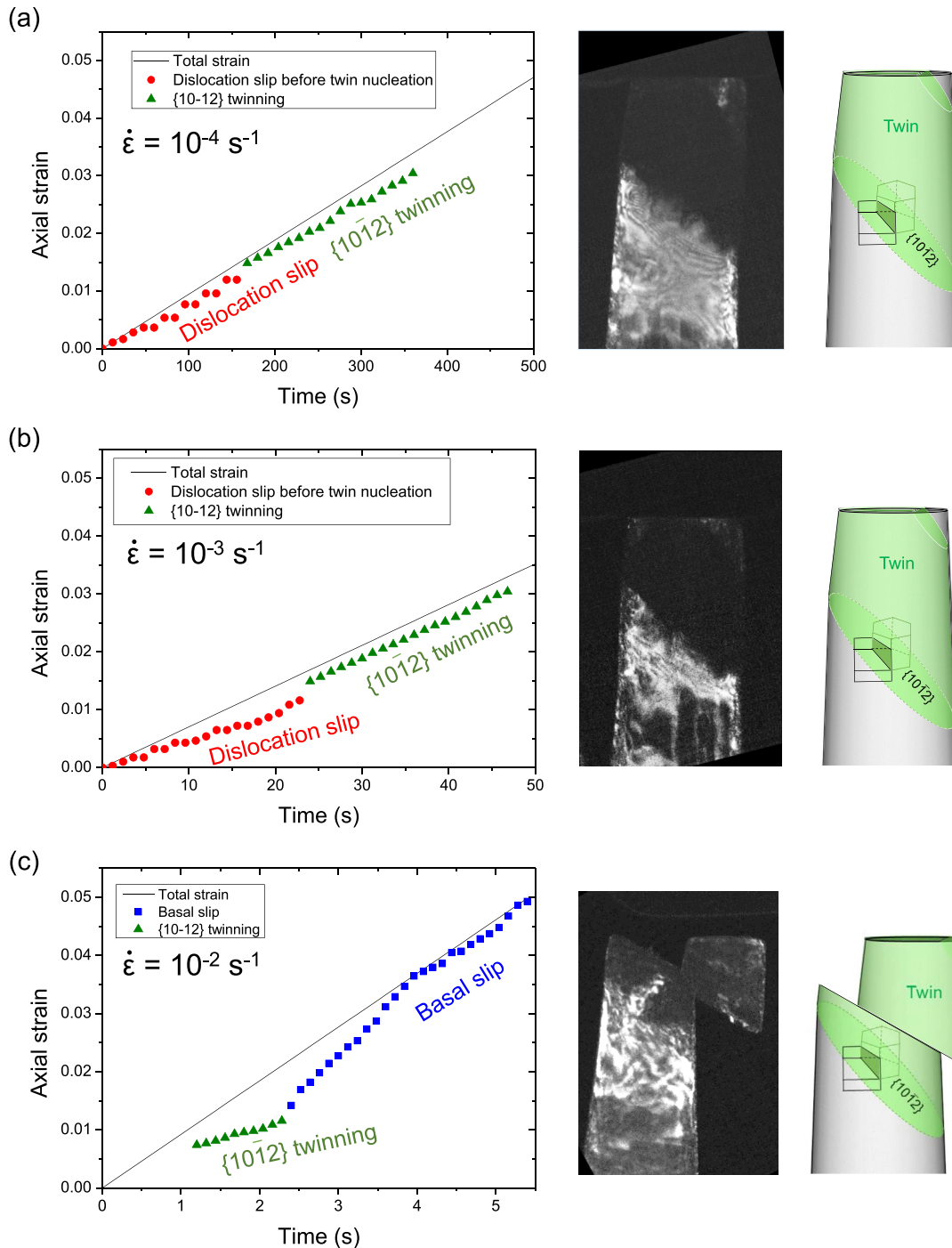
Fig. 13. Tracing of the axial strain of 0.5 \mu\text{m} Mg [2\bar{T}T0] pillars with deformation time during microcompression in the TEM at various strain rates. Plot of axial strain vs. time at the strain rate of: (a) 10^{-4} \text{ s}^{-1} ; (b) 10^{-3} \text{ s}^{-1} ; (c) 10^{-2} \text{ s}^{-1} . The applied strain is shown as straight line. The axial strain measured using frame images of TEM movies is indicated by symbol in each plot. Different symbols and colors are used to distinguish different deformation mode, e.g., red circles for dislocation slip, green triangles for \{10\bar{1}2\} twinning and blue squares for the basal slip within the twin. For each strain rate a TEM image and schematic are shown to represent the dominant deformation mode. The corresponding in-situ TEM movie and strain analysis are provided as Supplementary Movie S9, S10 and S11 for the strain rate of 10^{-4} \text{ s}^{-1} , 10^{-3} \text{ s}^{-1} , and 10^{-2} \text{ s}^{-1} , respectively. (For interpretation of the references to color in this figure legend, the reader is referred to the Web version of this article.)
