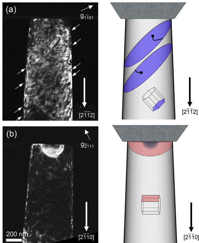
Fig. 6. TEM images and schematics representing the difference between basal \langle a \rangle and prismatic \langle a \rangle slip in the [2\bar{1}12] and the [2\bar{1}10] pillars during compression, respectively. (a) Mg [2\bar{1}12] pillar, where the basal plane is oriented favorable for dislocation slip. Several single-armed sources are activated, leading to local basal \langle a \rangle slip. The corresponding in-situ TEM movie is provided as Supplementary Movie S5 . (b) Mg [2\bar{1}10] pillar, where the prismatic plane is oriented favorable for dislocation slip (the pillar of interest in this paper). Different from the easy activation of basal slip in the Mg [2\bar{1}12] pillar, dislocation half-loops emanating from a source in the Mg [2\bar{1}10] pillar are non-glissile, leading to the formation of a strongly localized strain contour (refer to Fig. 7).
