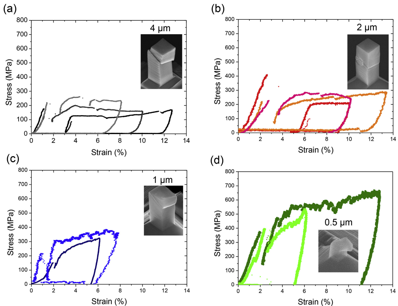
Fig. 2. Stress-strain curves of Mg [2\bar{1}\bar{1}0] pillars with sizes of (a) 4\text{ }\mu\text{m} ; (b) 2\text{ }\mu\text{m} ; (c) 1\text{ }\mu\text{m} ; (d) 0.5\text{ }\mu\text{m} . A representative SEM image of deformed pillar is shown for each size as inset.
