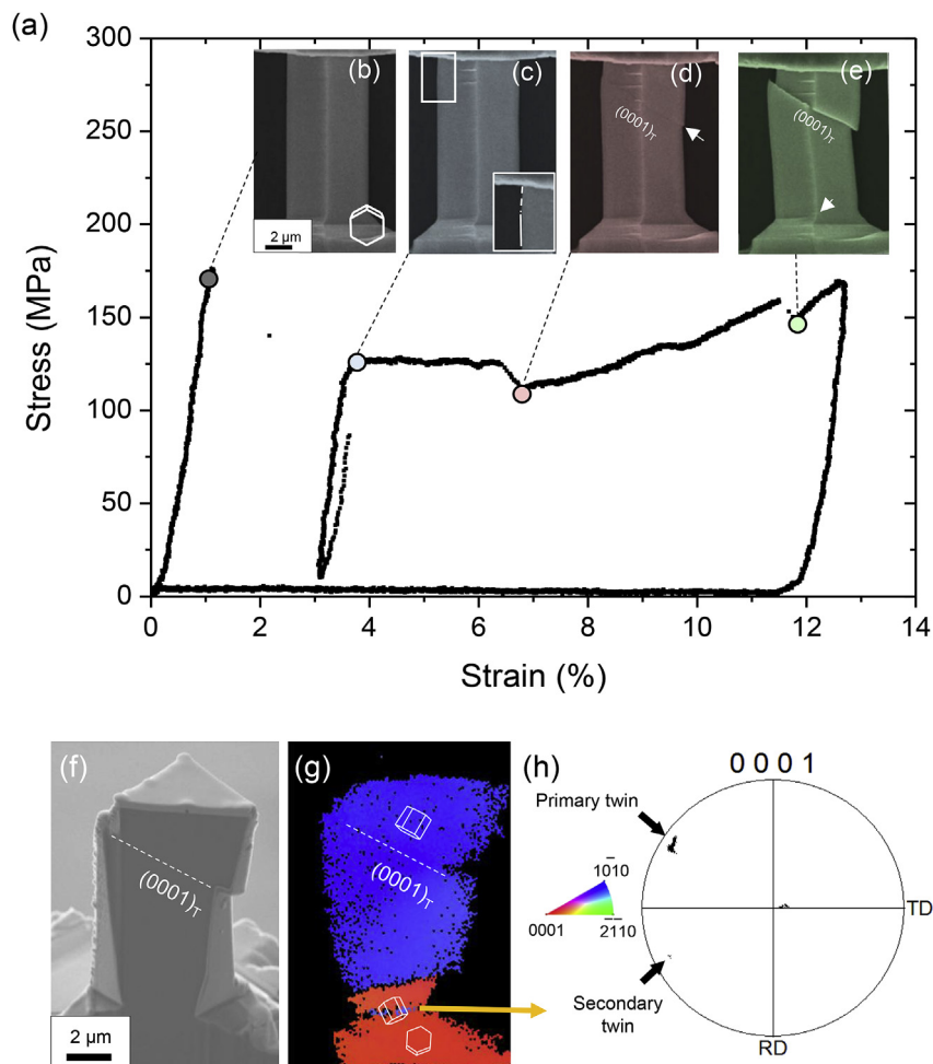
Fig. 1. In-situ SEM microcompression results of a 4 \mu\text{m} Mg [2\bar{1}\bar{1}0] pillar at a strain rate of 10^{-3} \text{ s}^{-1} . (a) Stress-strain curve. (b–e) SEM images corresponding to the positions marked on the stress-strain curve. In specific, (b) before onset of plastic deformation ( \epsilon = 1.1\% ); (c) after the large load drop ( \epsilon = 3.7\% ) showing a tilt of the sample edge due to {10 \bar{1}2 } twinning; (d) formation of a slip line along the (0001)_T basal plane (white arrow) within the twinned region ( \epsilon = 6.5\% ); (e) activation of the secondary twin at the base of pillar (white arrow) ( \epsilon = 11.5\% ). The in-situ SEM movie with correlated stress-strain curve is provided as Supplementary Movie S1 . (f) Cross-section of the deformed pillar prepared by FIB. (g) EBSD orientation map of the cross-section. (h) EBSD (0001) pole figure showing the formation of two {10 \bar{1}2 } twin variants indicated as primary and secondary twins.
