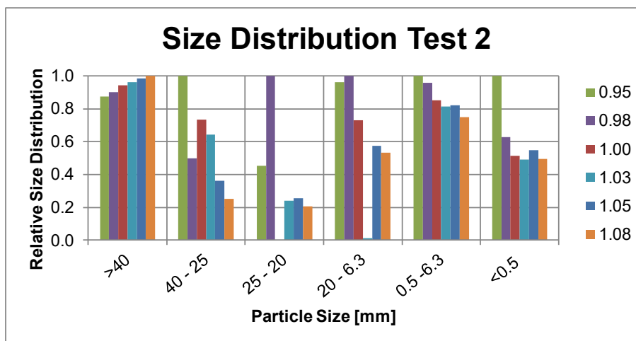
Figure 64: Size distribution of Test 2 after tumble test with relative press torque set points from 0.95 to 1.08
