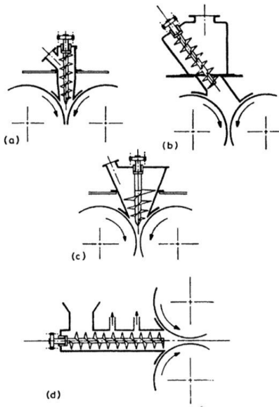
Figure 16: Some typical screw feeders: (a) vertical straight or slightly tapered screw feeder, (b) inclined straight screw feeder, (c) vertical tapered screw feeder, (d) horizontal straight screw feeder [23]
