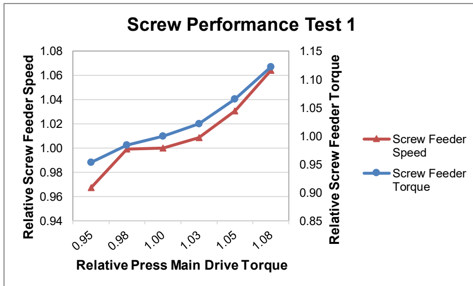
Figure 67: Screw performance Test 1
