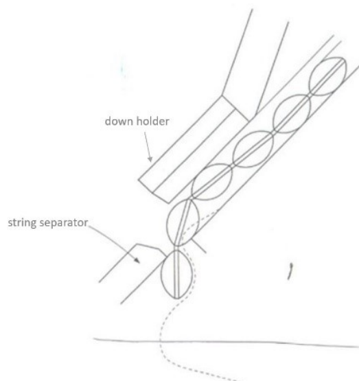
Figure 19: Schematic representation of the briquetting string separation [28]
