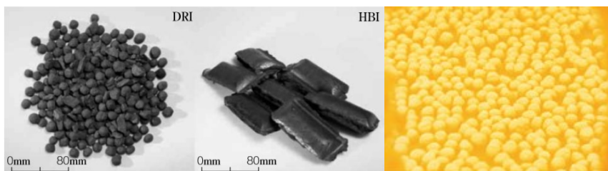
Figure 1: Cold DRI (CDRI), Hot Briquetted Iron (HBI) and Hot DRI (HDRI) [7], [8]
