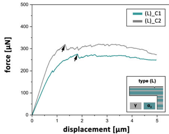
Figure 4: Force–displacement data of cantilevers exhibiting their expected crack propagation plane perpendicular to the \alpha_2/\gamma lamellae. Therein, distinct force drops without simultaneous crack growth are marked by arrows, indicating the positions of respective data points from Table 2.
