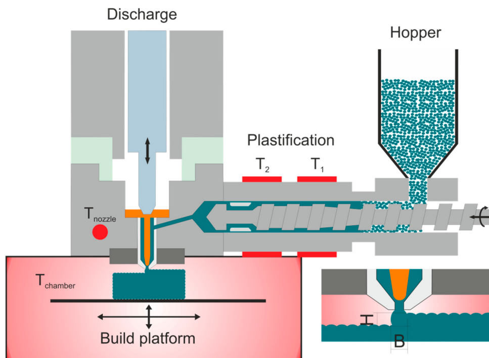
Figure 1. Working principle of Arburg Plastic Freeforming process where T_1 is the temperature in cylinder zone 1, T_2 is the temperature in cylinder zone 2, T_{nozzle} is the nozzle temperature, and T_{chamber} is the chamber temperature. B and H are the width and height of the produced droplets, respectively.
