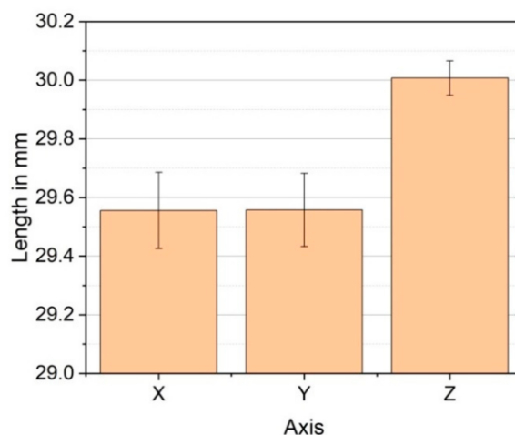
Figure 8. Shrinkage in each printing direction for cubic specimens 30\text{ mm} \times 30\text{ mm} \times 30\text{ mm} .
