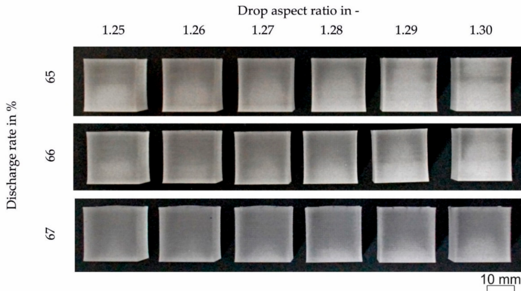
Figure 7. Cubic specimens printed at different discharge rates (65, 66 and 67%) and drop aspect ratios between 1.25 and 1.30. Other processing temperatures were T_1 = 200\text{ }^{\circ}\text{C} , T_2 = 230\text{ }^{\circ}\text{C} , T_{\text{nozzle}} = 245\text{ }^{\circ}\text{C} , and T_{\text{chamber}} = 100\text{ }^{\circ}\text{C} .
