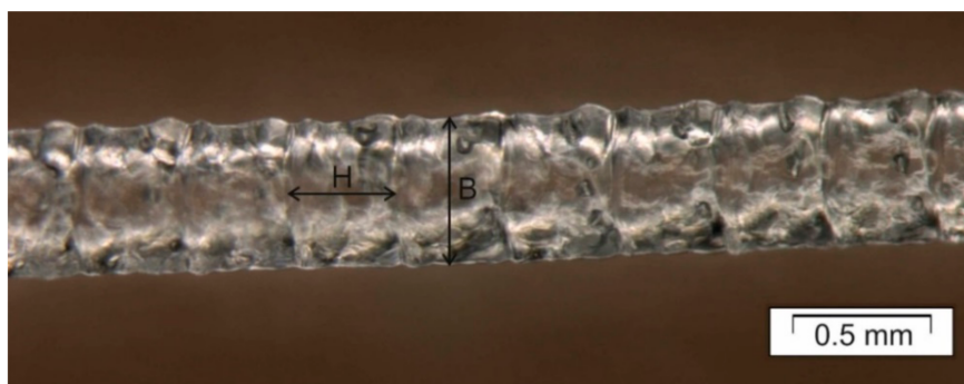
Figure 2. Micrograph of a string of droplets obtained using the initial printing conditions in Table 2. H values are from 0.22 to 0.25 mm and B values from 0.28 to 0.32 mm, giving a drop aspect ratio (DAR = B/H) of approximately 1.26.
