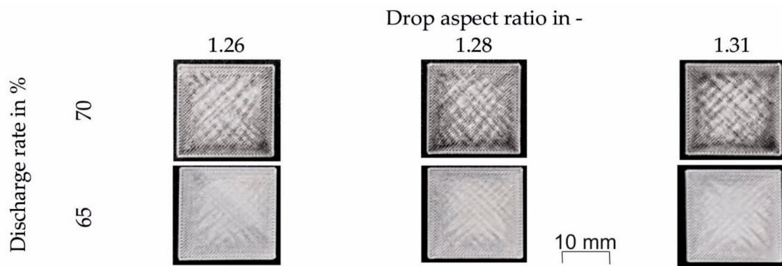
Figure 4. Cubic specimens printed at a chamber temperature of 100 °C with three different drop aspect ratios (1.26, 1.28, and 1.31) and discharge rates of 70 and 65%. Other processing temperatures were T_1 = 195 °C, T_2 = 225 °C, and T_{\text{nozzle}} = 240 °C.
