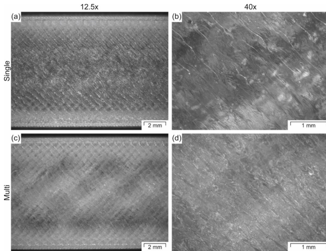
Figure 12. Microscopy images of tensile specimens printed in (a,b) batch of one specimen (Single) or (c,d) five specimens (Multi) recorded at two different magnifications (12.5 and 40). All images were taken from the top view and laying the specimens in the XY-plane.
