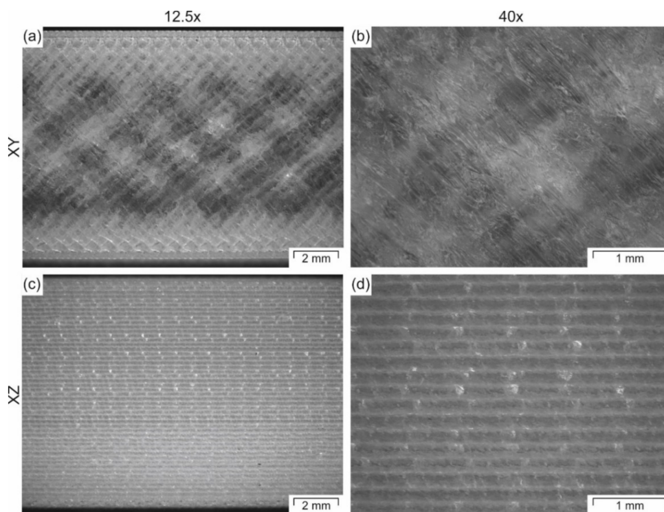
Figure 11. Microscopy images of tensile specimens printed in (a,b) XY-orientation or (c,d) XZ-orientation recorded at two different magnifications (12.5 and 40). All images were taken from the top view and laying the specimens in the XY-plane.
