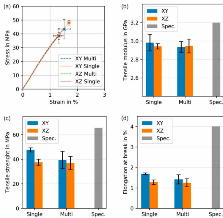
Figure 10. Tensile mechanical properties of printed specimens in two orientations (XY and XZ) and the batch of one specimen (Single) or five specimens (Multi): (a) stress-strain curves, (b) tensile modulus, (c) tensile strength, and (d) elongation at break. Specifications (Spec.) for the neat (most likely injection molded PMMA) given by the producer are given for comparison. Individual stress-strain curves can be seen in the Supplementary Information (Figure S1).
