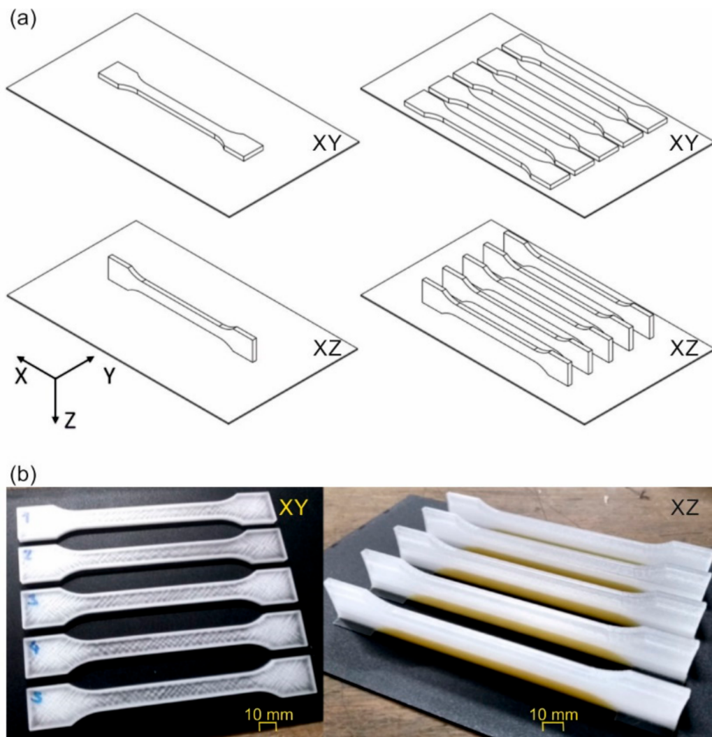
Figure 3. (a) Schematic representation of different orientations (XY or XZ) and arrangements (single or multiple) of tensile bars during printing, and (b) examples of printed parts without support material and with support material (yellowish material).
