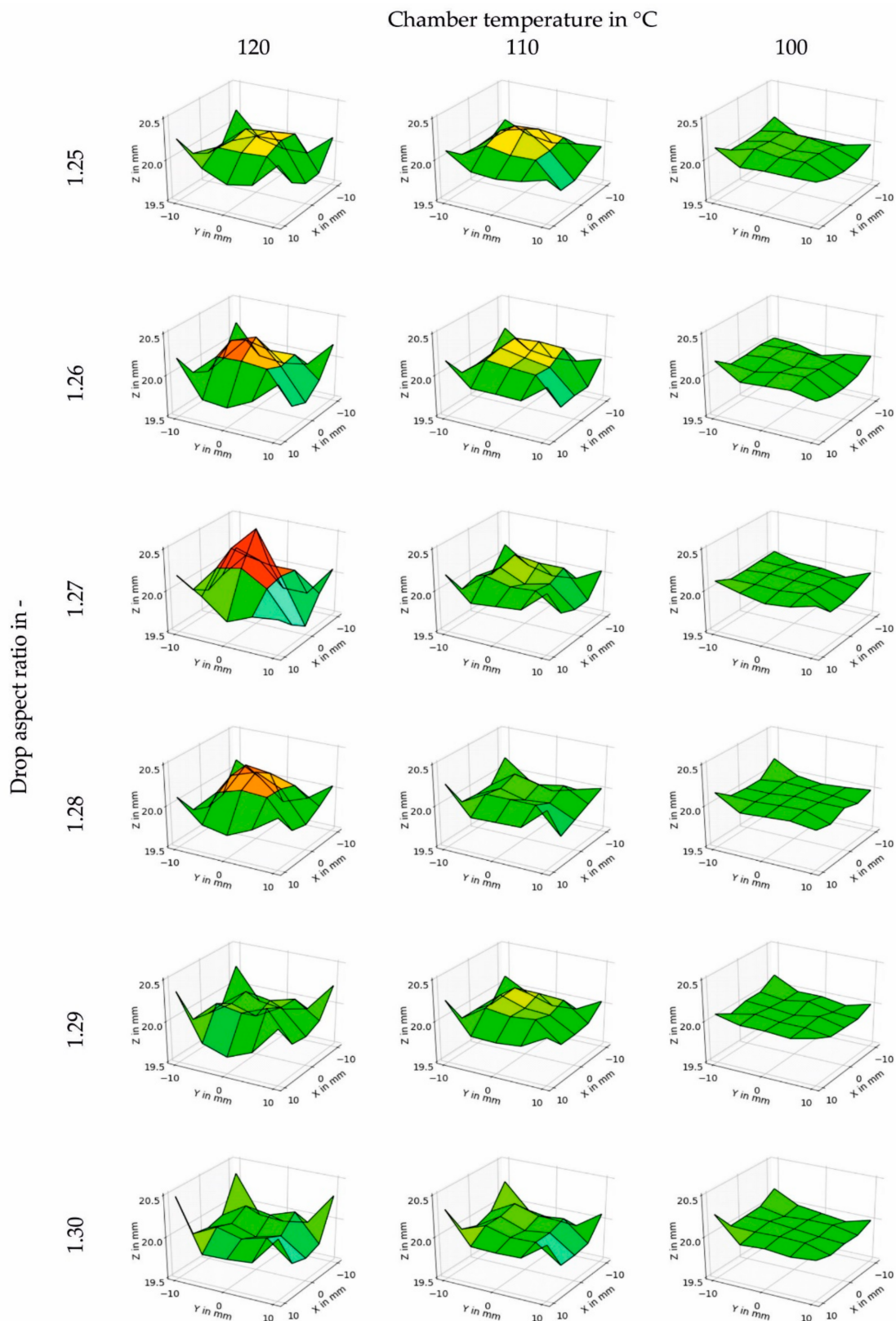
Figure 6. Surface plots of the height measured for cubic specimens printed at different chamber temperatures between 120 and 100 °C and different drop aspect ratios between 1.25 and 1.30. Other processing temperatures were T_1 = 200 °C, T_2 = 230 °C, and T_{\text{nozzle}} = 245 °C.
