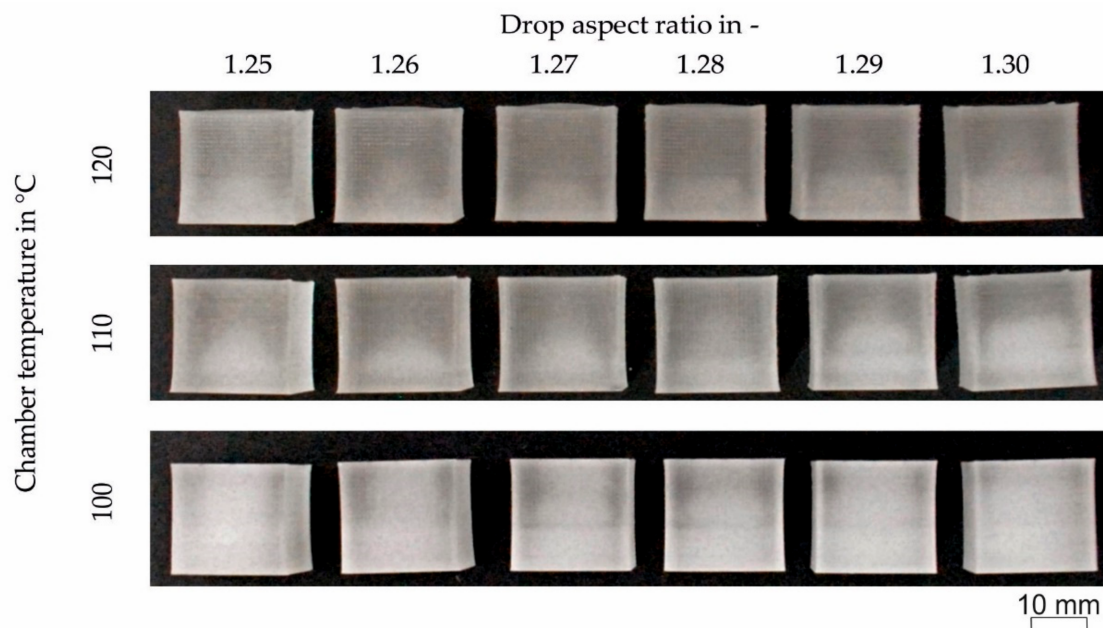
Figure 5. Printed cubes with six different values for the drop aspect ratio between 1.25 and 1.30, and three different chamber temperatures ( T_{\text{chamber}} ) and decreased drop overlap of 25%. Other processing temperatures were T_1 = 200 °C, T_2 = 230 °C, and T_{\text{nozzle}} = 245 °C.
