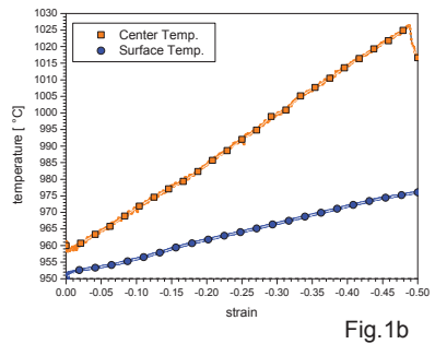
Fig. 1: Measured temperature evolution in the center and on the surface of the specimen for a target temperature of 950°C and for strain rates of 0.1 s -1 (a) and 10 s -1 (b). Fig. 2: Measured signals of a stress relaxation test with the initial surface temperature of 1050°C of the specimen at a logarithmic strain of 0.3 and a strain rate of 10 s -1 (a) and at pre-strains of 0.10, 0.15, ..., 0.30 (b).
