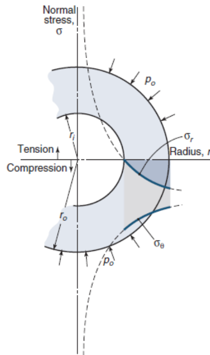
Figure 62: Radial and circumferential stress behavior for different radii for an externally pressurized, thick-walled cylinder; Source: (Schmid, S.R.; Hamrock, B. J.; Jacobson 2014)
