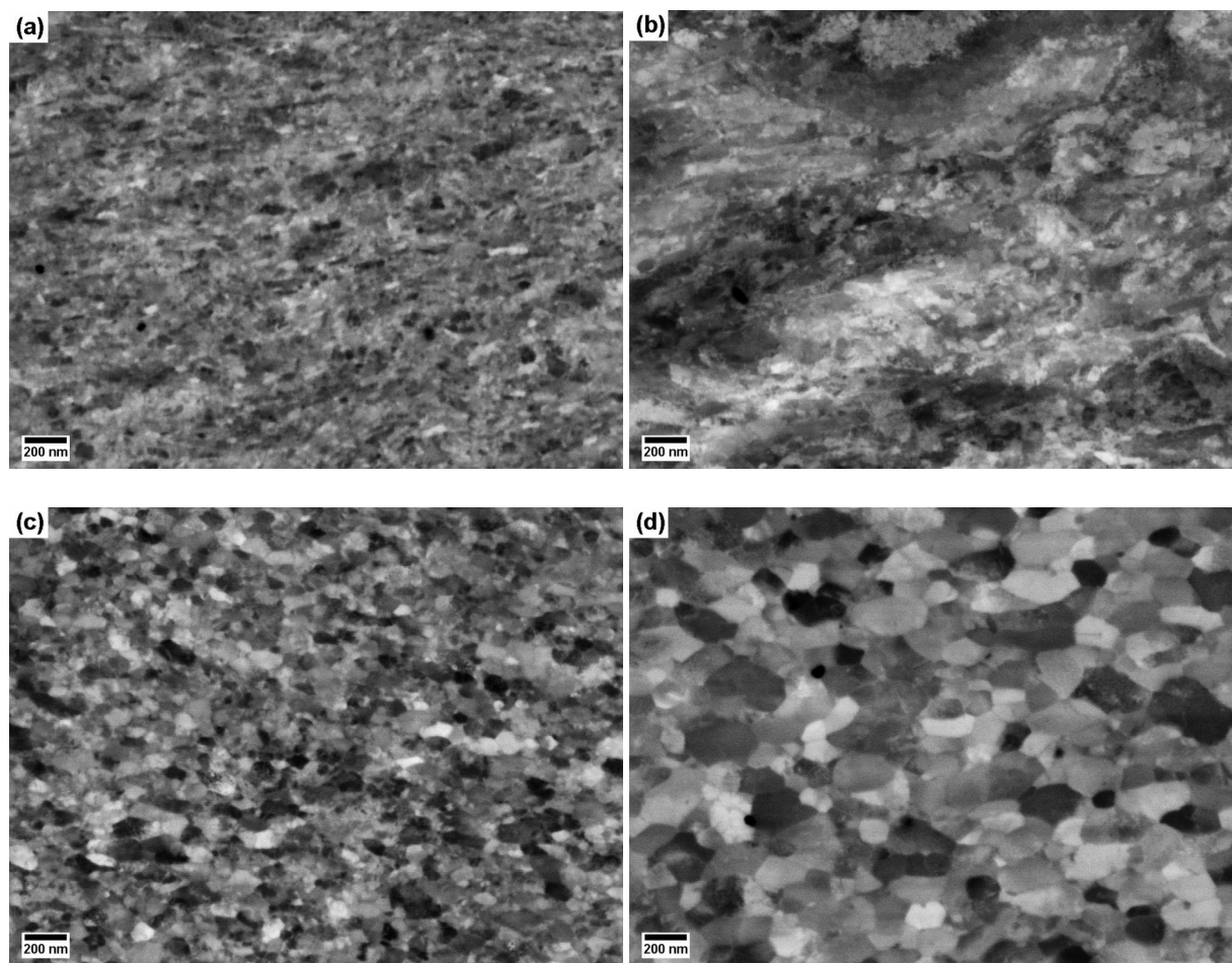
Figure C1: SEM micrographs after HPT at (a) room temperature, (b) 200 °C, (c) 350 °C and (d) 450 °C at radius r = 3 mm (1 revolution, \epsilon_{VM} = 15 ).
