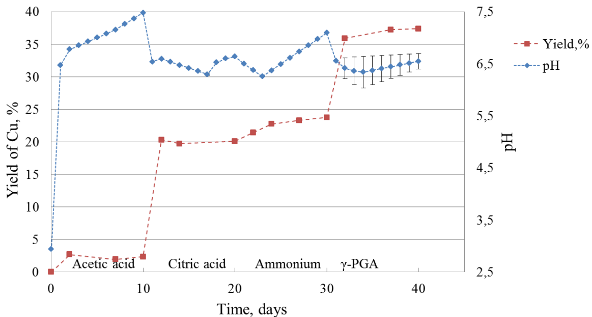
Figure 37 Leaching kinetics of Rudna Carbonate with stepwise change of supernatant
