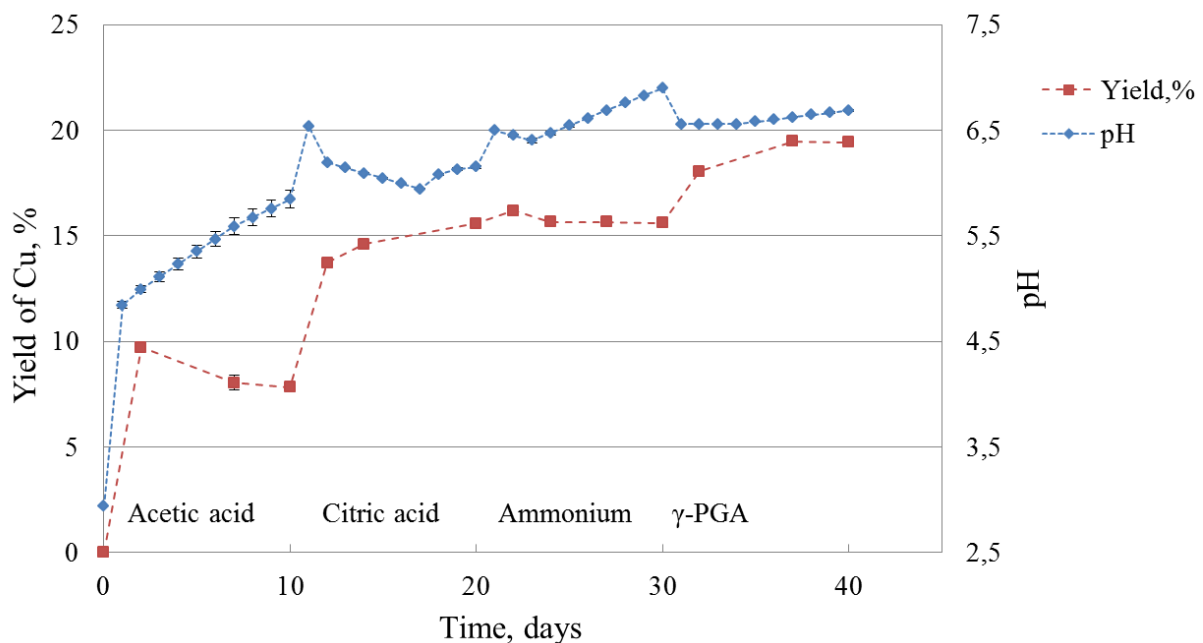
Figure 24 Leaching kinetics of Sangerhausen copper shale with stepwise change of supernatant
