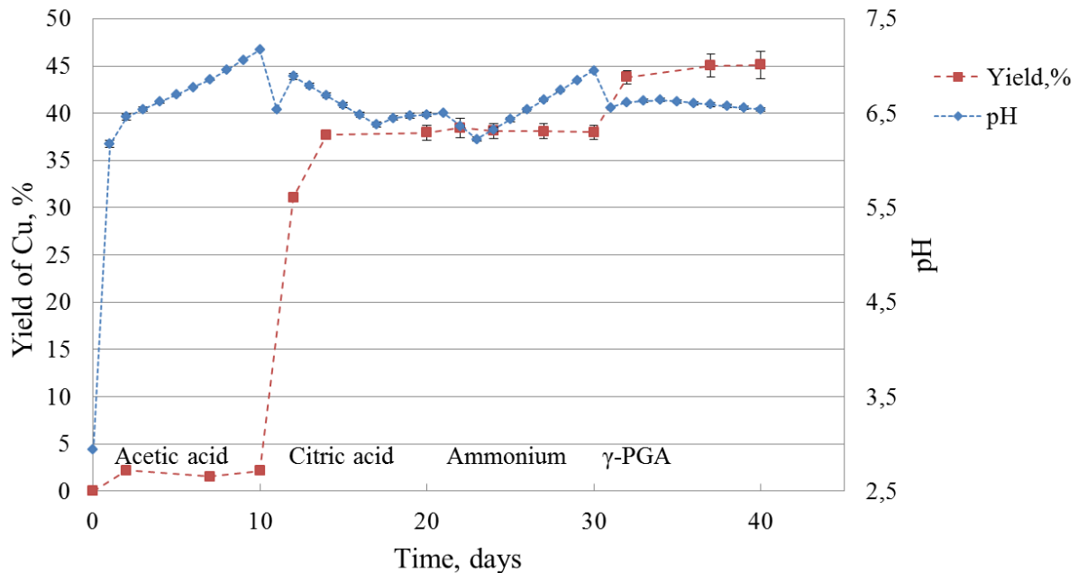
Figure 20 Leaching kinetics of Mansfeld Copper shale (slime) with stepwise change of supernatant
