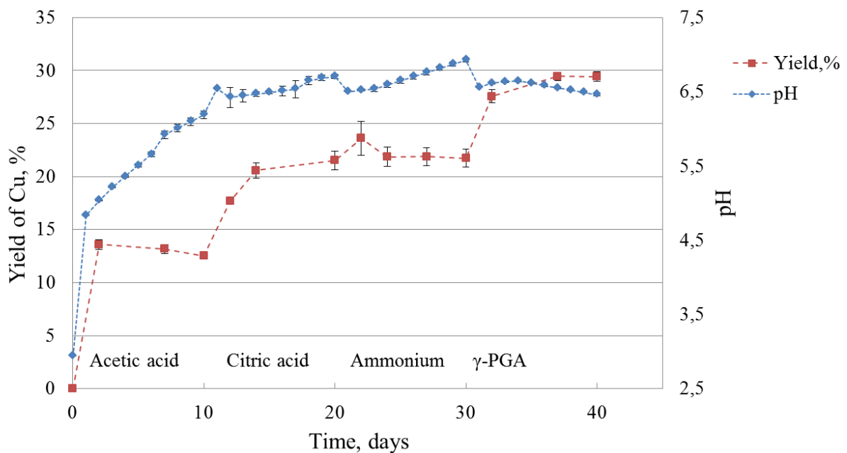
Figure 15 Leaching kinetics of Mansfeld Copper shale (deslimed) with stepwise change of supernatant
