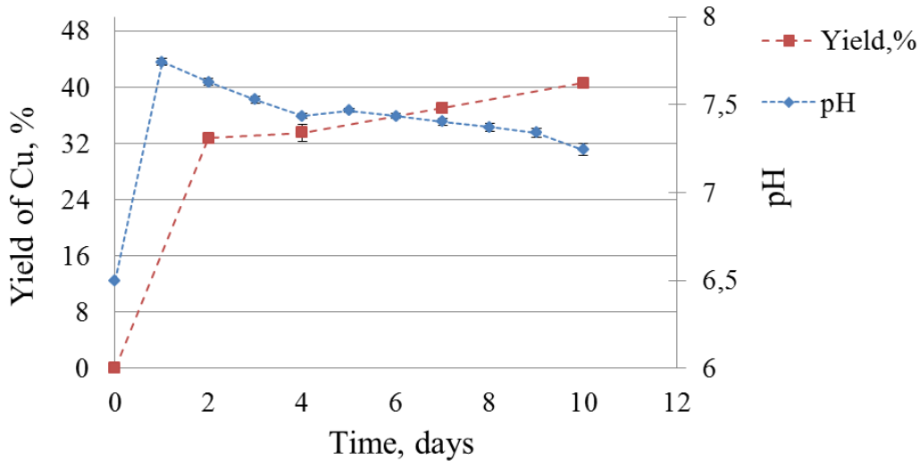
Figure 18 Leaching kinetics of Mansfeld copper shale (slime) by PGA
