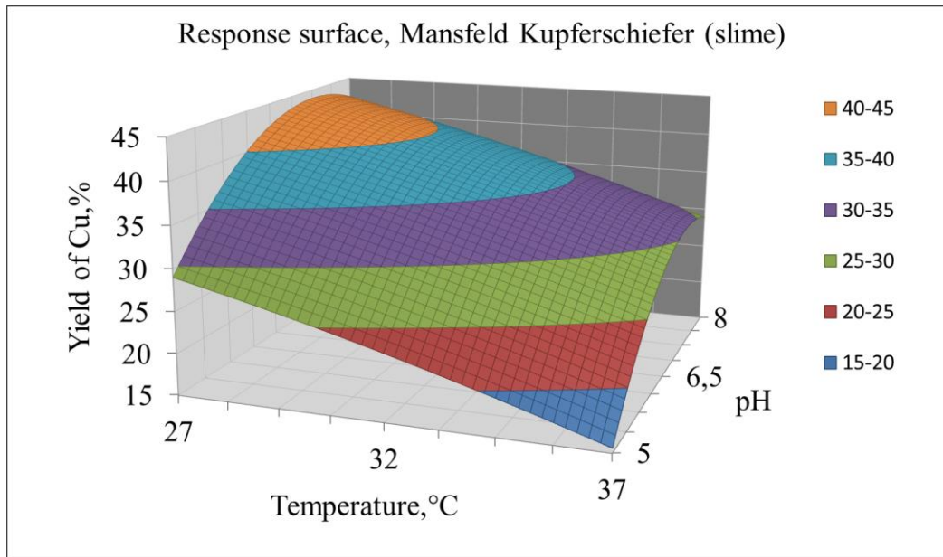
Figure 19 Response surface model for Mansfeld copper shale (slime)
