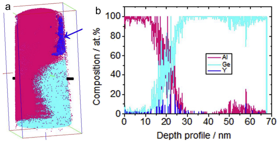
Fig. 9. (a) 3D reconstructions of eutectic Al (pink), represented by iso-concentration surface at a threshold of 75 at% Al and eutectic Ge (cyan) represented by iso-concentration surface at a threshold of 90 at% Ge in the Al–20Ge–0.2Y alloy. The investigated volume is 75 \times 74 \times 154 \text{ nm}^3 . A Y-rich region is visualized by an iso-concentration surface at a threshold of 20 at%, as marked by a blue arrow. (b) Concentration depth profiles across the interface between eutectic Al and eutectic Ge along the cylinder (indicated in (a)) with a radius of 1.5 nm. (For interpretation of the references to colour in this figure legend, the reader is referred to the web version of this article.)
