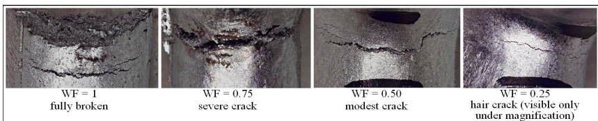
Figure 2. WF for various hot cracking levels [21,22].
