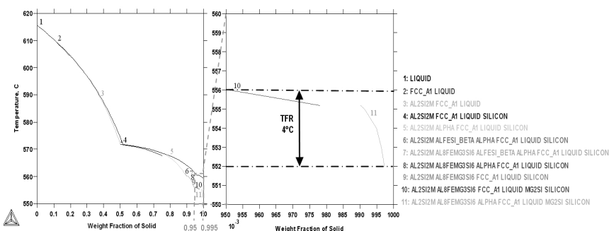
Figure 7. TCC, calculation of TFR (4°C), AlSi7Mg0.6Cu0.05.
