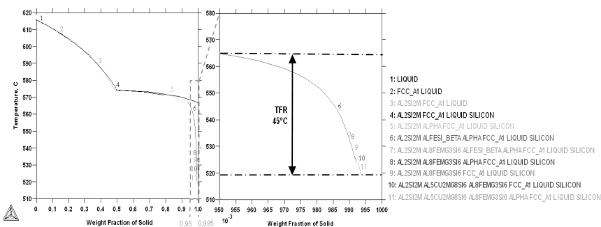
Figure 6. TCC, calculation of TFR (45°C), AlSi7Mg0.1Cu0.5.
