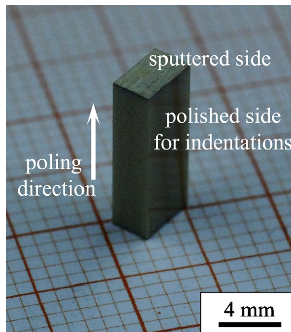
Fig. 1. Bulk PZT specimen showing the sputtered surfaces, the polished surfaces and the direction of poling.
