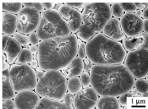
Fig. 2. SEM micrograph of the microstructure of the PZT bulk material. A random alignment of domains can be seen within the grains.
