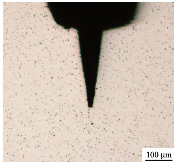
Fig. 5. Pre-notched PZT bulk specimen for fracture toughness determination.
